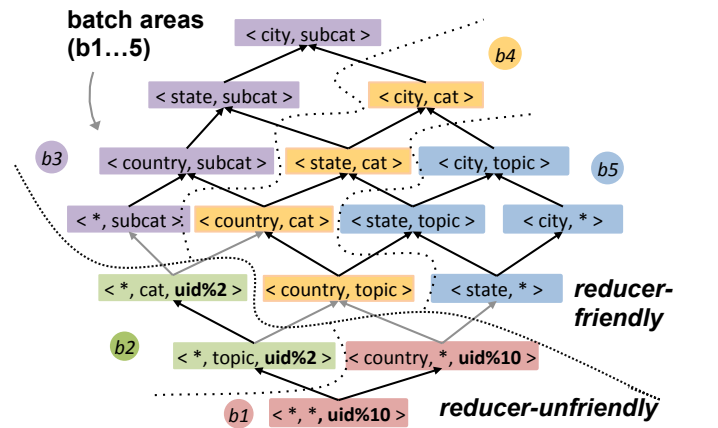
Fig. 9. Annotated Cube Lattice. Each color in the lattice indicates a batch area, b_1 ... b_5 . The reducer-friendly blocks are grouped into three batch areas to exploit pruning and reduce intermediate data size. Two of the reducer-unfriendly regions are value partitioned on uid into 10 partitions.
